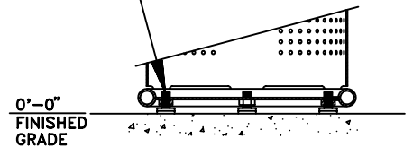
2615-FT-L (LEVELING MOUNT) SCALE: 3/4"=1'-0"
