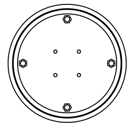
2615-FT-P (PEDESTAL MOUNT) SCALE: 3/4"=1'-0"
