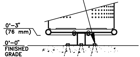
2615-FT-P (PEDESTAL MOUNT) SCALE: 3/4"=1'-0"
